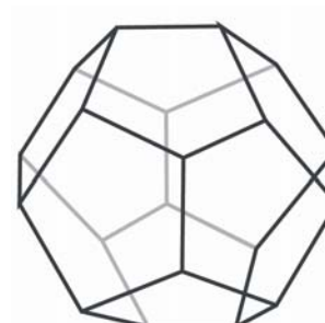
dodecahedron
