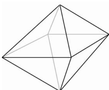
octahedron
